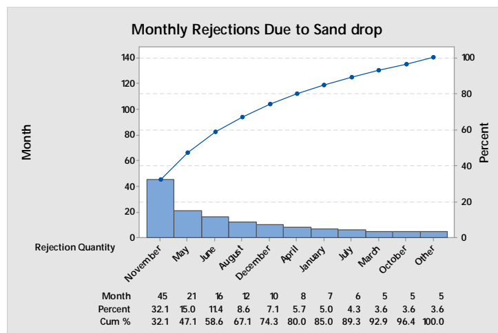
Fig. 3- Pareto Diagram for Monthly Rejections due to Sand Drop Defect
