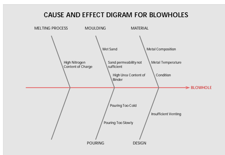
Fig. 2-Cause and Effect Diagram for Blowhole Defect
