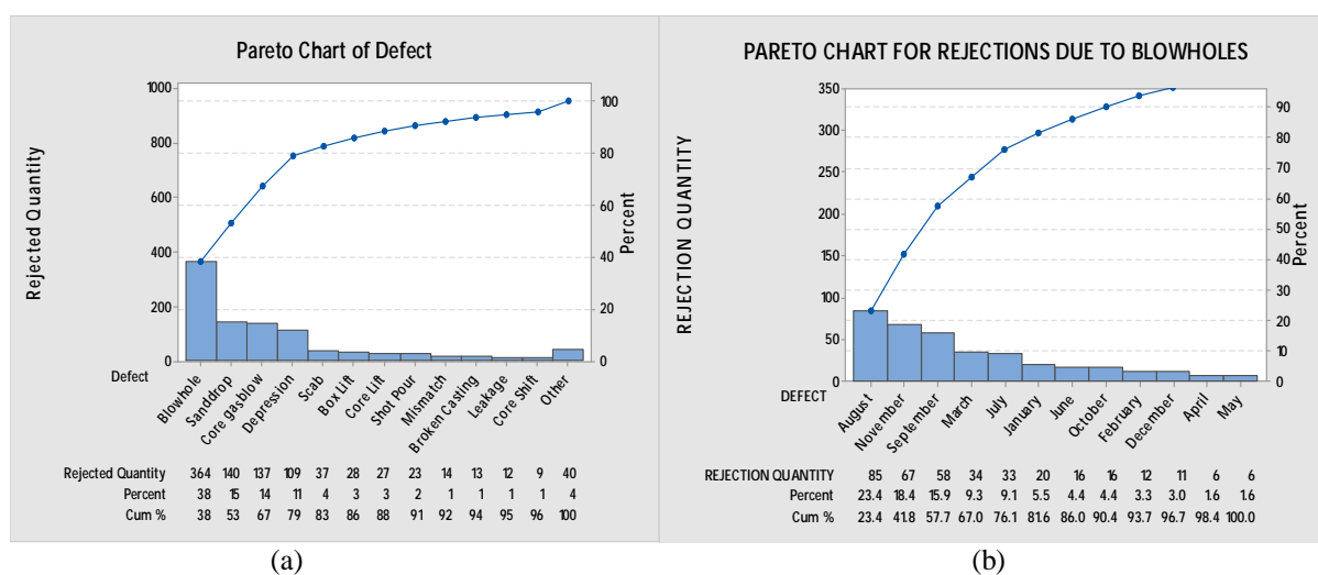
Fig. 1 Pareto charts for the defects (a) Pareto Chart for overall rejections due to various defects (b) Pareto Chart for defects due to Blowholes
